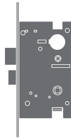
EURO Mortise Lock
