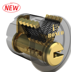
CYL- SK D01 13-pin three way key cylinder
