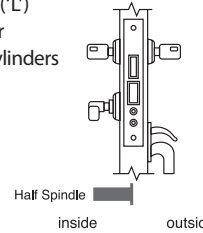
4628-A2 Entrance / Apartment ('DTK') With Knobs Double Cylinders
