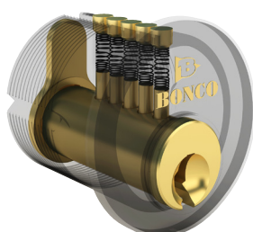
CYL-D01 regular 5-pin key cylinder
