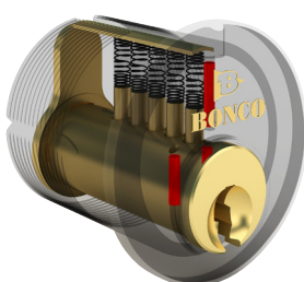
CYL- NS D01 regular 5-pin key with prevent drill bar cylinder
