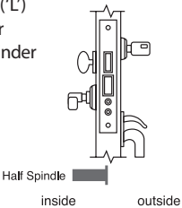
4628-A1 Entrance / Apartment ('DTK') With Knobs Single Cylinder
