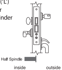
4628-A1 Entrance / Apartment ('DTK') With Knobs Single Cylinder
