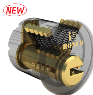
CYL- SKD 01 13-pin three way key cylinder
