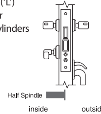
4628-A2 Entrance / Apartment ('DTK') With Knobs Double Cylinders
