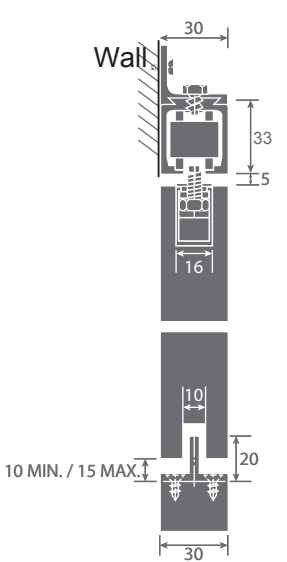
Side Wall Fixing Only For DT-081C
