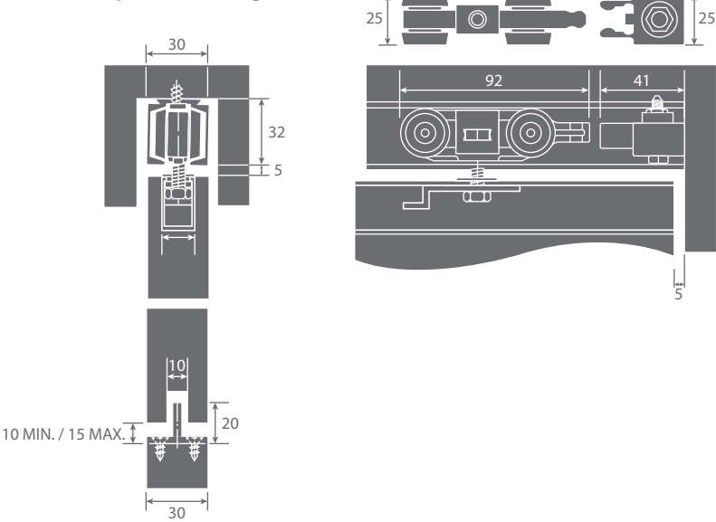
Top Jamb Fixing
