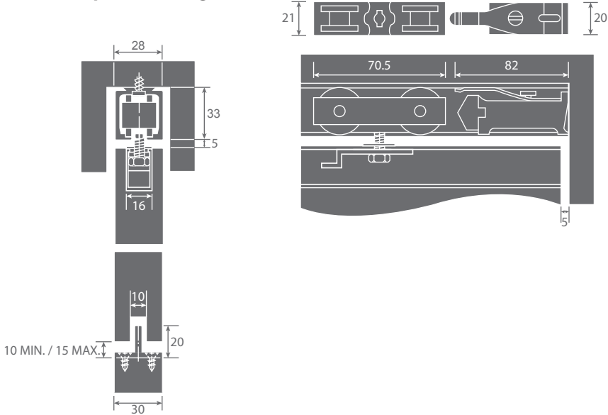
Top Jamb Fixing
