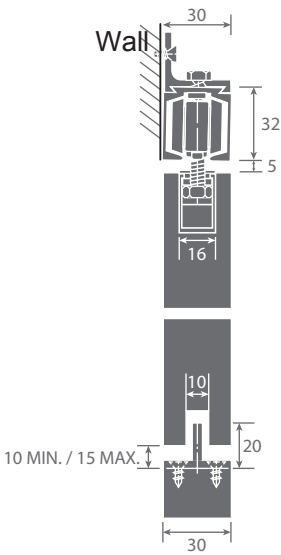
Side Wall Fixing Only For DT-052C
