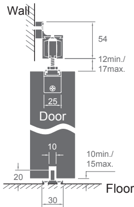
Side Wall Fixing (Only for DT-052T)
