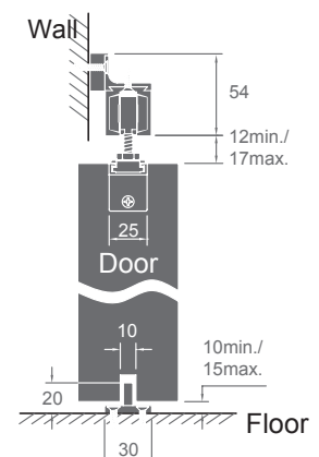
Side Wall Fixing (Only for DT-052T)
