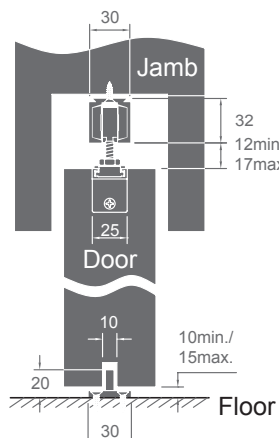
Top Jamb Fixing
