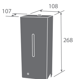
MSD12R/ 22R/ 32R NEW
