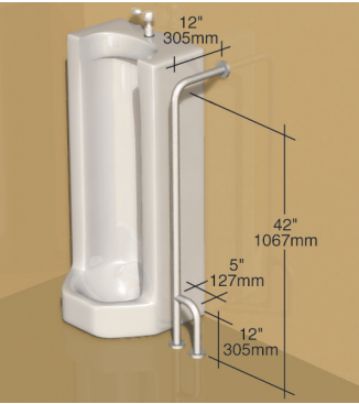
122RH Floor to wall with outrigger
