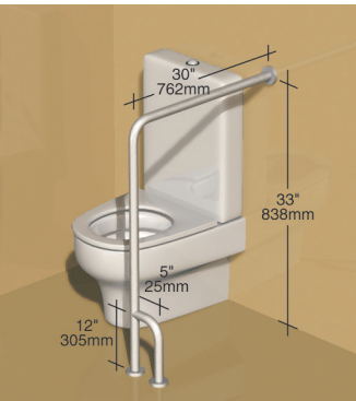
133RH Wall to floor with outrigger
