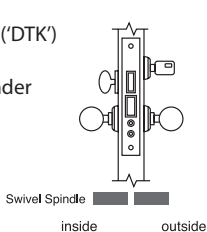
4628-B1 Entrance / Apartment ('DTL') With Levers Single Cylinder
