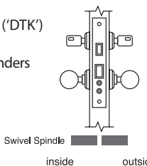
4628-B2 Entrance / Apartment ('DTL') With Levers Double Cylinders
