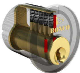
CYL- NS D01 regular 5-pin key with prevent drill bar cylinder
