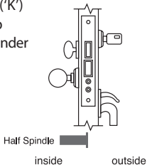
4627-B1 Entrance ('L') With Lever Single Cylinder
