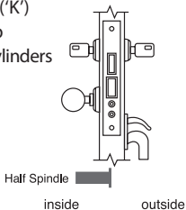
4627-B2 Entrance ('L') With Lever Double Cylinders
