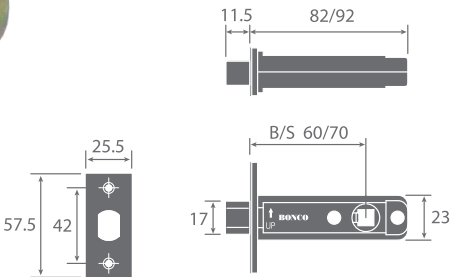
Face Plate (Stainless Steel)
