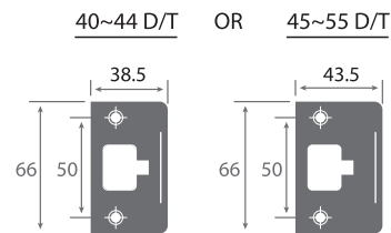
Strike Plate (Stainless Steel)
